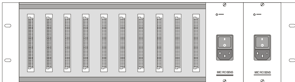
3HU Chassis (MS416001M) with two power supplies for redundancy (MS416004M):
